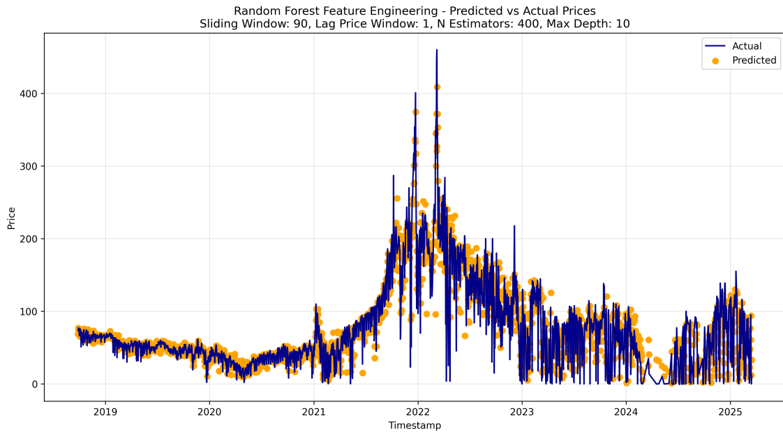
Fig. 4.8. Best Random Forest feature engineering model
