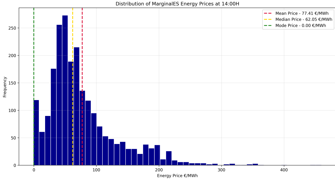
Fig. 4.2. MarginalES at 14:00H Data Distribution, Including Mean, Median and Mode Values
